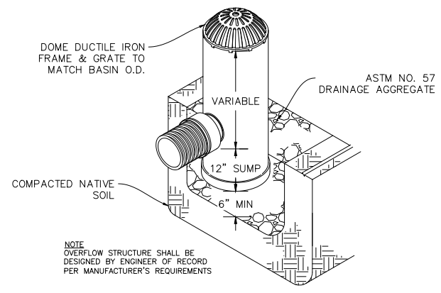
OVERFLOW STRUCTURE
