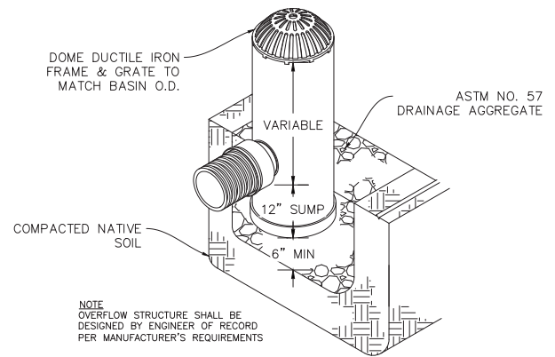
OVERFLOW STRUCTURE
