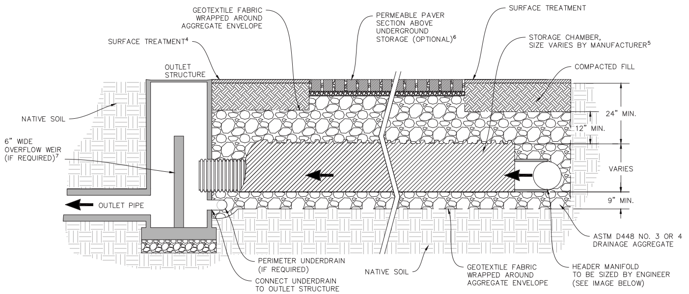
UNDERGROUND STORAGE SECTION
