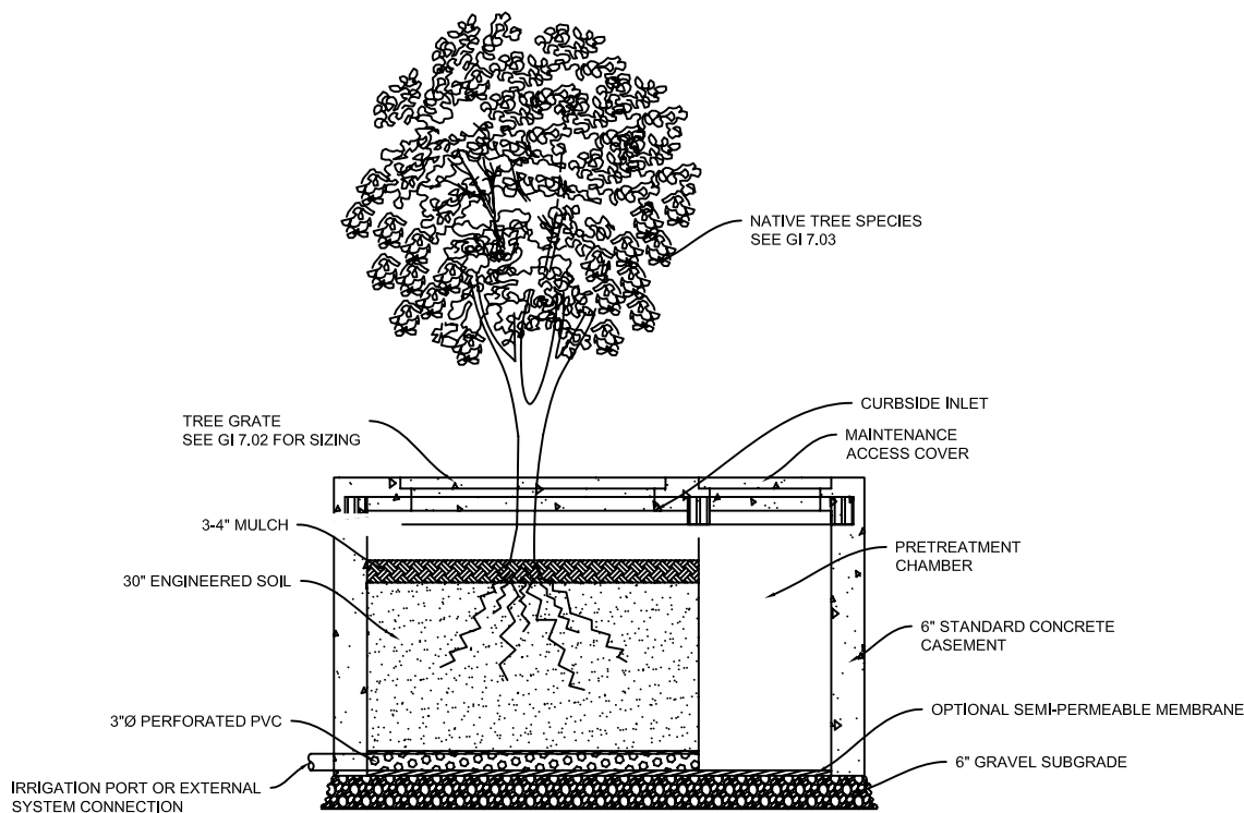
BOX TREE FILTER TYPICAL SECTION
