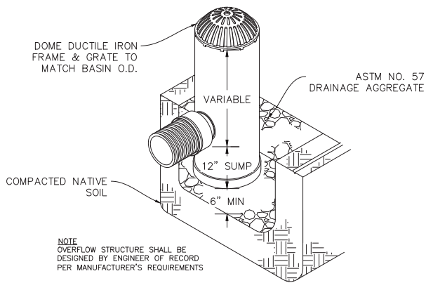
OVERFLOW STRUCTURE
