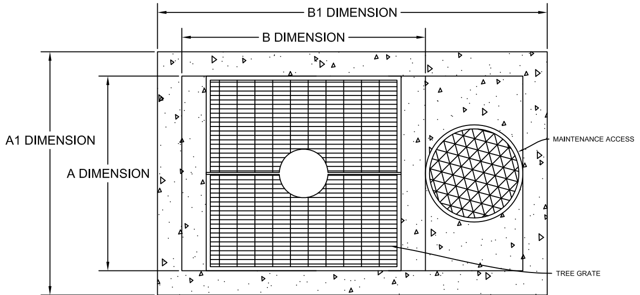
TOP VIEW AND SIZE SELECTION DETAIL
