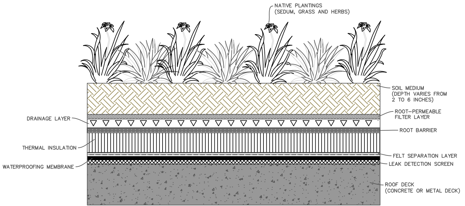
GREEN ROOF TYPICAL SECTION
